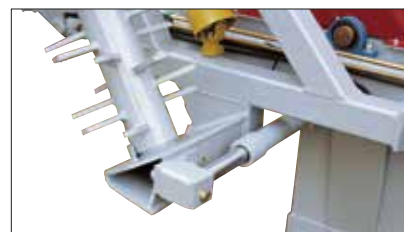
Separate hydraulic folding cylinders are standard equipment.
