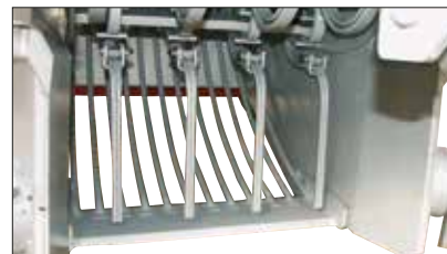
The collecting drum of SB4000 has a rotor with 18 and SB5200 24 Kongskilde tines.
