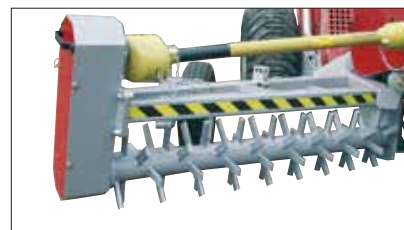
The Stone rake collects the stones to the drum.
